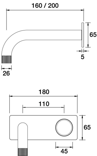
IDK Vetro Wall Bath Mixer Set 200mm outlet Incl. plate A48.041.2.54 - Volcanic Grey
