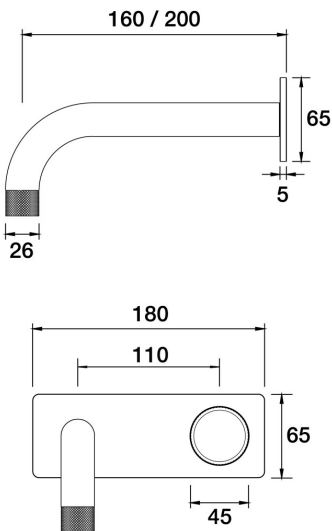
IDK Vetro Wall Bath Mixer Set 200mm outlet Incl. plate A48.041.2.67 - Vintage Brass
