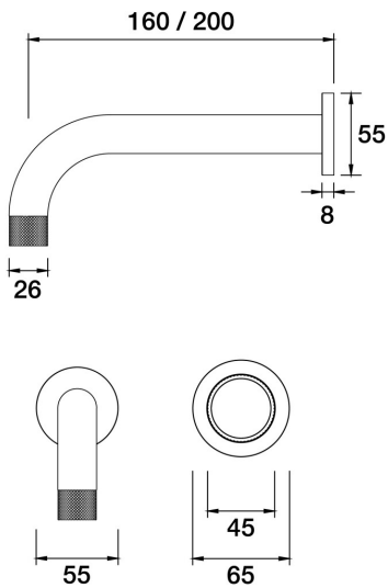
IDK Vetro Wall Bath Mixer Basin Set. 200mm outlet A48.043.2.52 - Burnished
