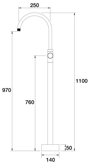
IDK Vetro Floor Bath Filler Mixer - Gooseneck A48.072.1.32 - Midnight Black
