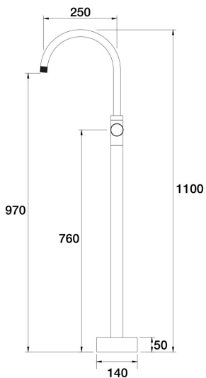
IDK Vetro Floor Bath Filler Mixer - Gooseneck A48.072.1.39 - Antique Bronze
