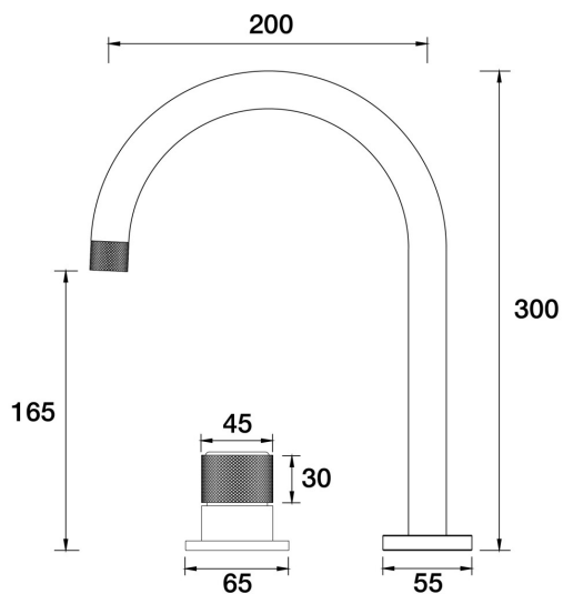
IDK Vetro Hob Mixer Set A48.081.3.19 - 23k Brushed Brass Gold
