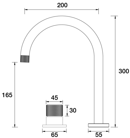
IDK Vetro Hob Mixer Set A48.081.3.57 - Matt Nickel
