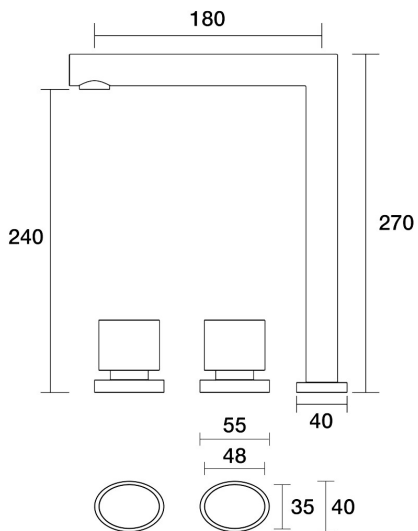
Oracle Basin Set Swivel B21.011.1.34 - Matt Black
