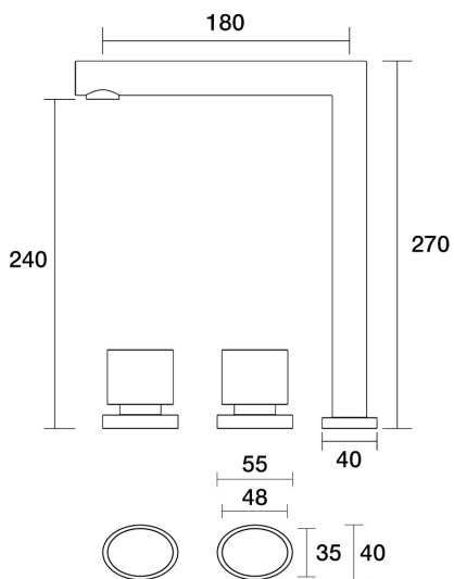
Oracle Sink Set Hob Swivel B21.051.1.02 - Brushed Chrome
