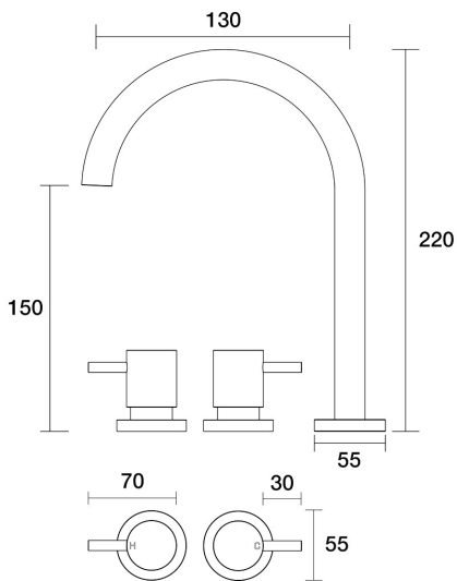
Lugano Basin Set Swivel B22.011.1.57 - Matt Nickel
