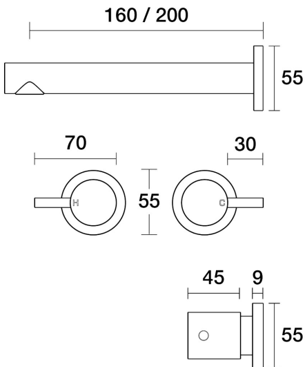
Lugano Wall Bath Set 160mm Outlet B22.021.1.02 - Brushed Chrome
