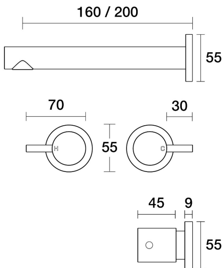
Lugano Wall Bath Set 160mm Outlet B22.021.1.23 - Gunmetal
