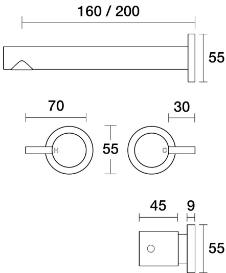
Lugano Wall Bath Set 160mm Outlet B22.021.1.67 - Vintage Brass
