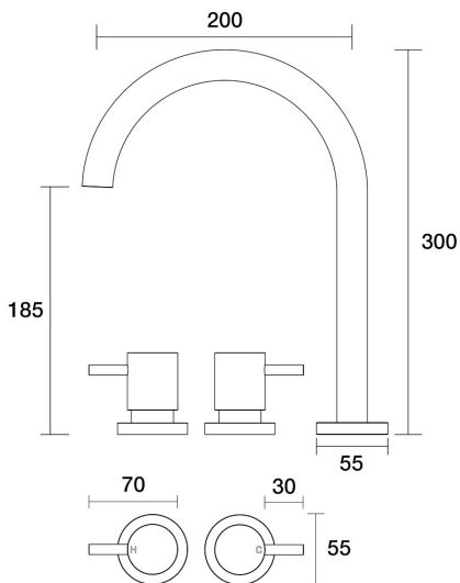
Lugano Sink Set Hob Swivel B22.051.1.45 - Native Brass
