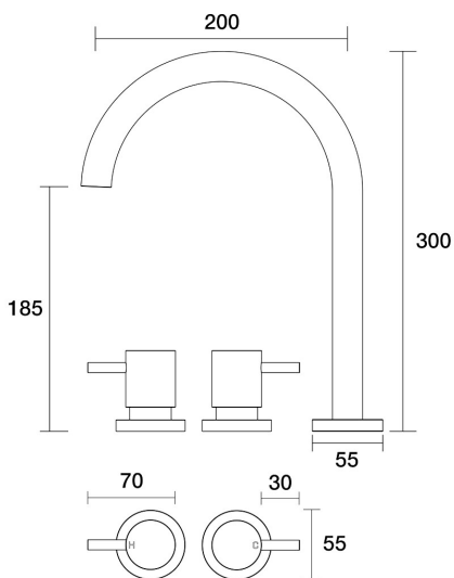
Lugano Spa Set Hob Swivel B22.061.1.24 - Brushed Gunmetal
