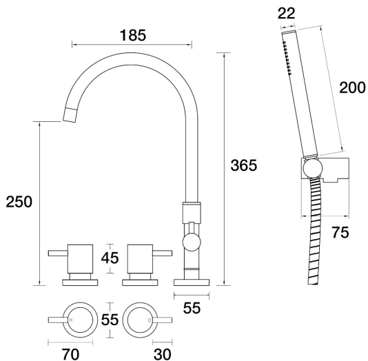
Lugano Spa Set Hob Swivel Divertor Set Gooseneck with Handshower & Bracket B22.061.5.25 - Brushed Nickel
