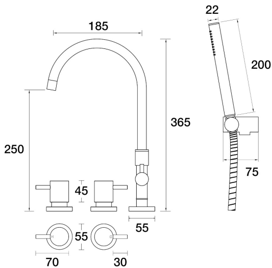
Lugano Spa Set Hob Swivel Divertor Set Gooseneck with Handshower & Bracket B22.061.5.34 - Matt Black
