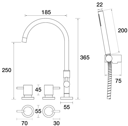
Lugano Spa Set Hob Swivel Divertor Set Gooseneck with Handshower & Bracket B22.061.5.39 - Antique Bronze
