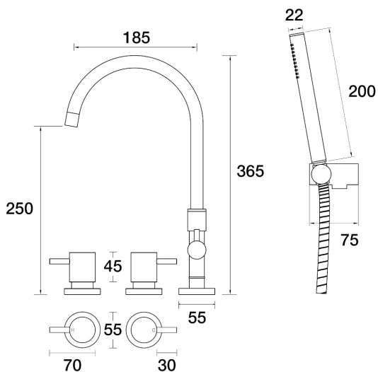
Lugano Spa Set Hob Swivel Divertor Set Gooseneck with Handshower & Bracket B22.061.5.42 - Brushed Copper
