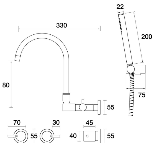
Lugano Spa Set Wall Swivel Divertor Set Gooseneck with Handshower & Bracket B22.062.5.01 - Chrome
