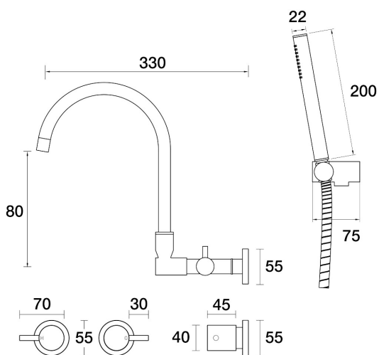
Lugano Spa Set Wall Swivel Divertor Set Gooseneck with Handshower & Bracket B22.062.5.42 - Brushed Copper
