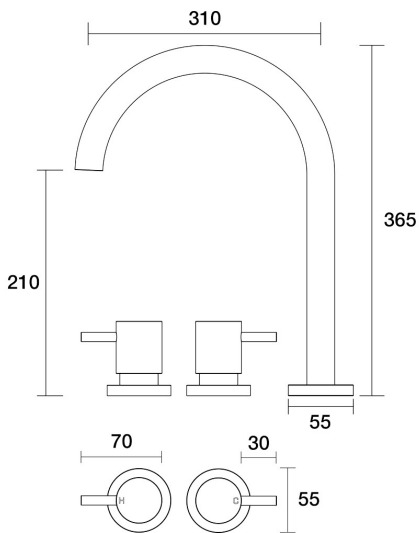
Lugano Spa Set XL Hob Swivel B22.063.1.48 - Copper
