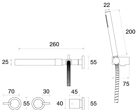
Lugano Spa Set Wall Fixed Divertor Set with Handshower & Bracket B22.065.1.01 - Chrome
