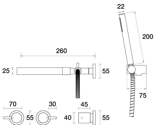
Lugano Spa Set Wall Fixed Divertor Set with Handshower & Bracket B22.065.1.02 - Brushed Chrome
