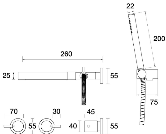
Lugano Spa Set Wall Fixed Divertor Set with Handshower & Bracket B22.065.1.47 - Luminick
