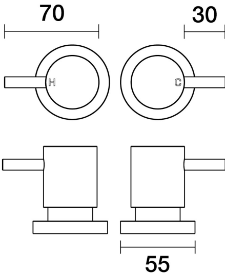
Lugano Top Assemblies Wall Pair B22.082.1.21 - Brushed Rose Gold
