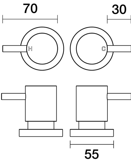
Lugano Top Assemblies Wall Pair B22.082.1.45 - Native Brass
