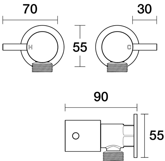
Lugano Washing Machine Stops Wall Pair B22.091.1.19 - 23k Brushed Brass Gold
