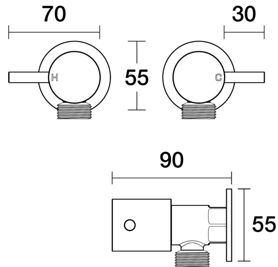
Lugano Washing Machine Stops Wall Pair B22.091.1.25 - Brushed Nickel
