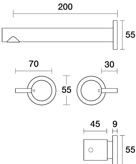
Lugano Wall Basin Set 200mm Outlet B22.152.1.12 - 23k Brushed Gold
