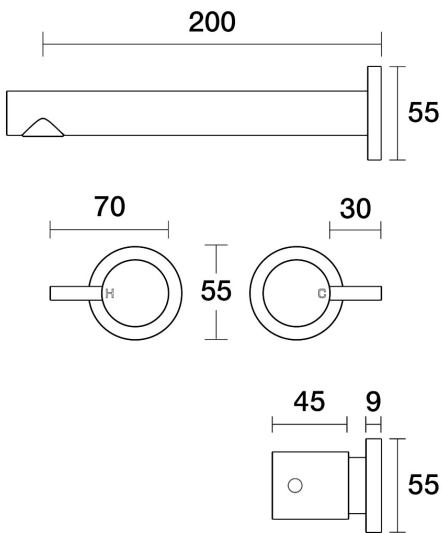
Lugano Wall Basin Set 200mm Outlet B22.152.1.41 - Brushed Brass
