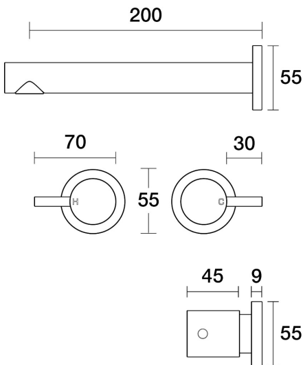
Lugano Wall Basin Set 200mm Outlet B22.152.1.42 - Brushed Copper
