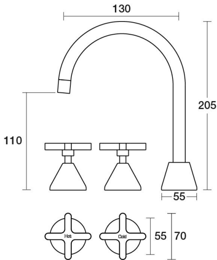
Forme Basin Set Swivel Ceramic Disc B27.011.2.01 - Chrome
