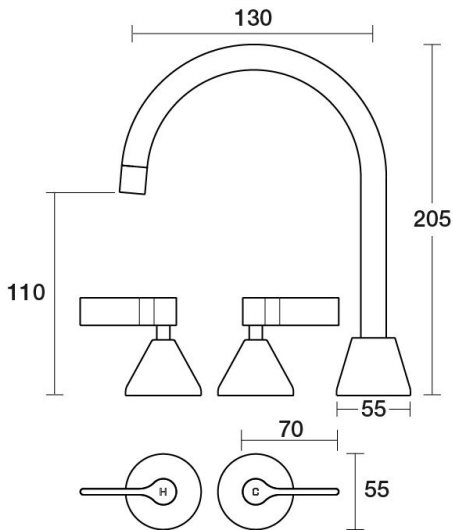
Forme Basin Set Swivel Lever Ceramic Disc B27.011.3.01 - Chrome
