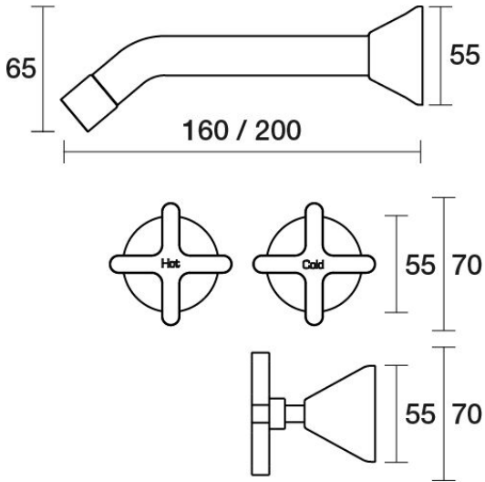
Forme Wall Bath Set 160mm Outlet B27.021.1.01 - Chrome
