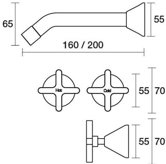
Forme Wall Bath Set 200mm Outlet B27.022.1.01 - Chrome
