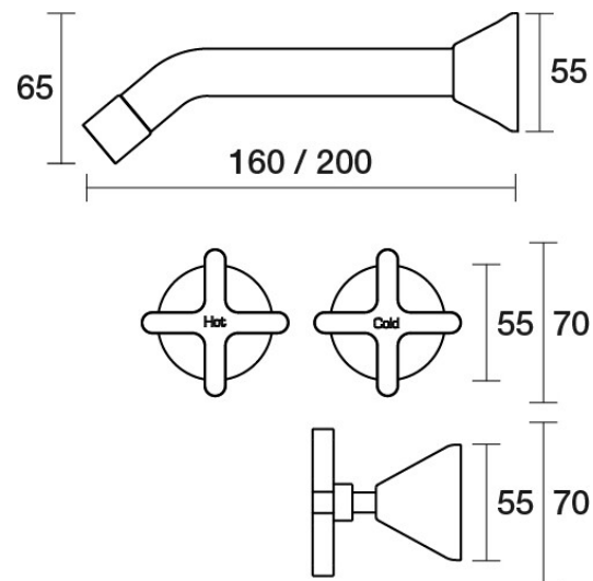
Forme Wall Bath Set 200mm Outlet B27.022.1.25 - Brushed Nickel
