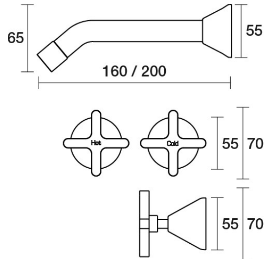
Forme Wall Bath Set 200mm Outlet B27.022.1.34 - Matt Black
