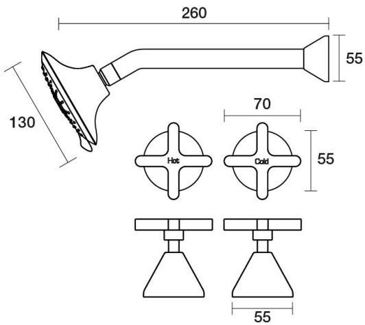
Forme Shower Set Fixed Arm B27.031.1.01 - Chrome
