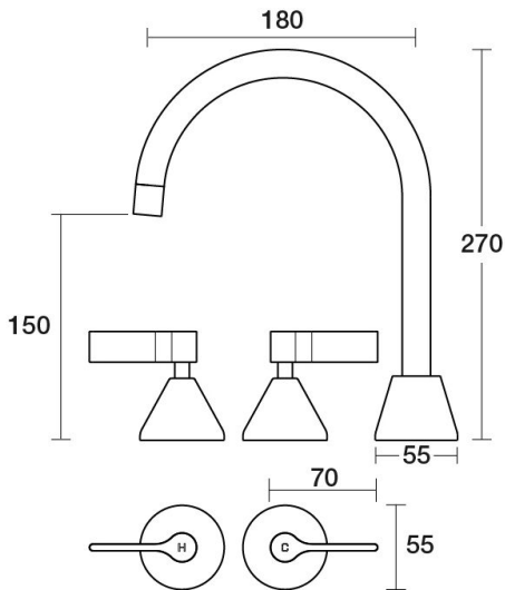
Forme Sink Set Hob Swivel Lever Ceramic Disc B27.051.3.01 - Chrome
