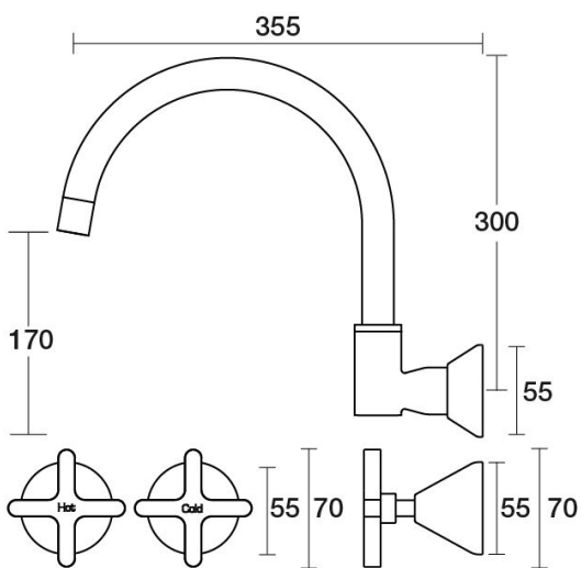
Forme Sink Set XL Wall Swivel Ceramic Disc B27.054.2.01 - Chrome
