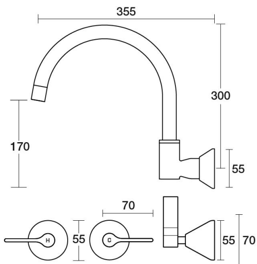
Forme - Online Exclusive Spa Set XL Wall Swivel Lever Ceramic Disc B27.064.3.01 - Chrome
