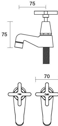
Forme Pillar Taps Pair B27.111.1.01 - Chrome
