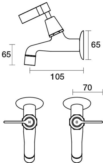
Forme Female Bibs Wall Pair Lever Ceramic Disc B27.121.3.01 - Chrome
