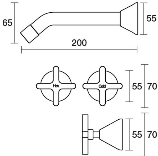
Forme Wall Basin Set 200mm Outlet B27.152.1.01 - Chrome
