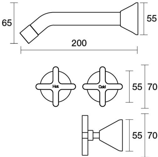
Forme Wall Basin Set 200mm Outlet Ceramic Disc B27.152.2.01 - Chrome
