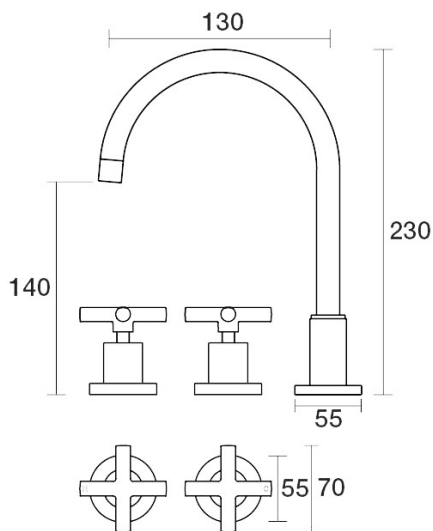
Portsea Basin Set Swivel Ceramic Disc B29.011.2.52 - Burnished
