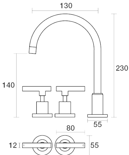
Portsea Basin Set Swivel Lever Ceramic Disc B29.011.3.01 - Chrome
