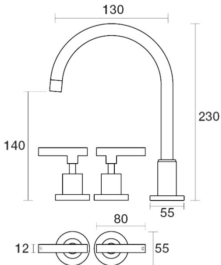
Portsea Basin Set Swivel Lever Ceramic Disc B29.011.3.45 - Native Brass
