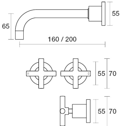
Portsea Wall Bath Set 160mm Outlet B29.021.1.26 - Black Sapphire
